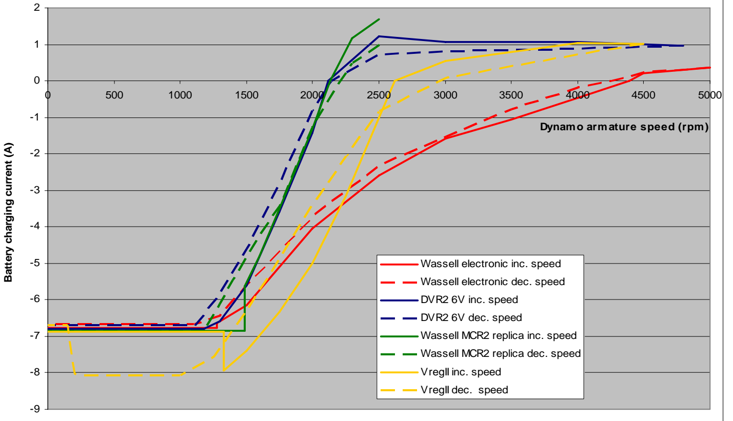
Battery Current with 42W light bulb load - 6V
